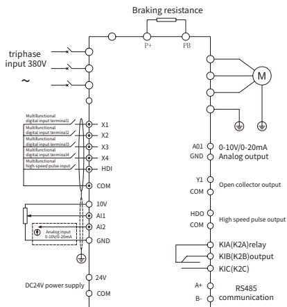
Fig 2-2 Wiring method of frequency converter control circuit
