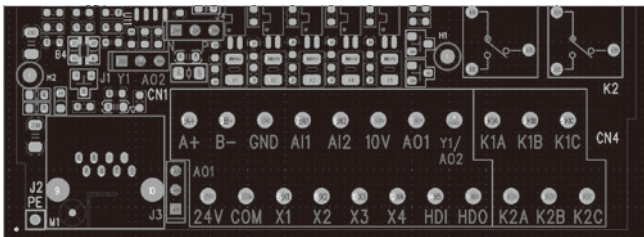
Fig 2-4 70 (isolated version) control circuit terminal layout
