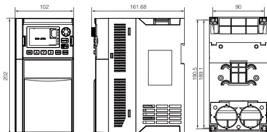
Profile size and installation size figure of 70 series plastic structure
