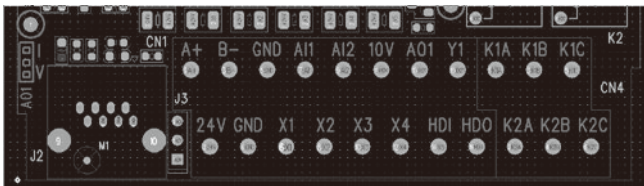
Fig 2-3 70(non isolated version) control circuit terminal layout
