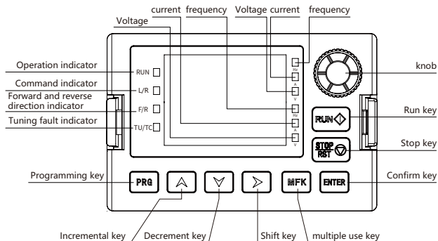
Fig 3-1 Schematic diagram of operation panel
